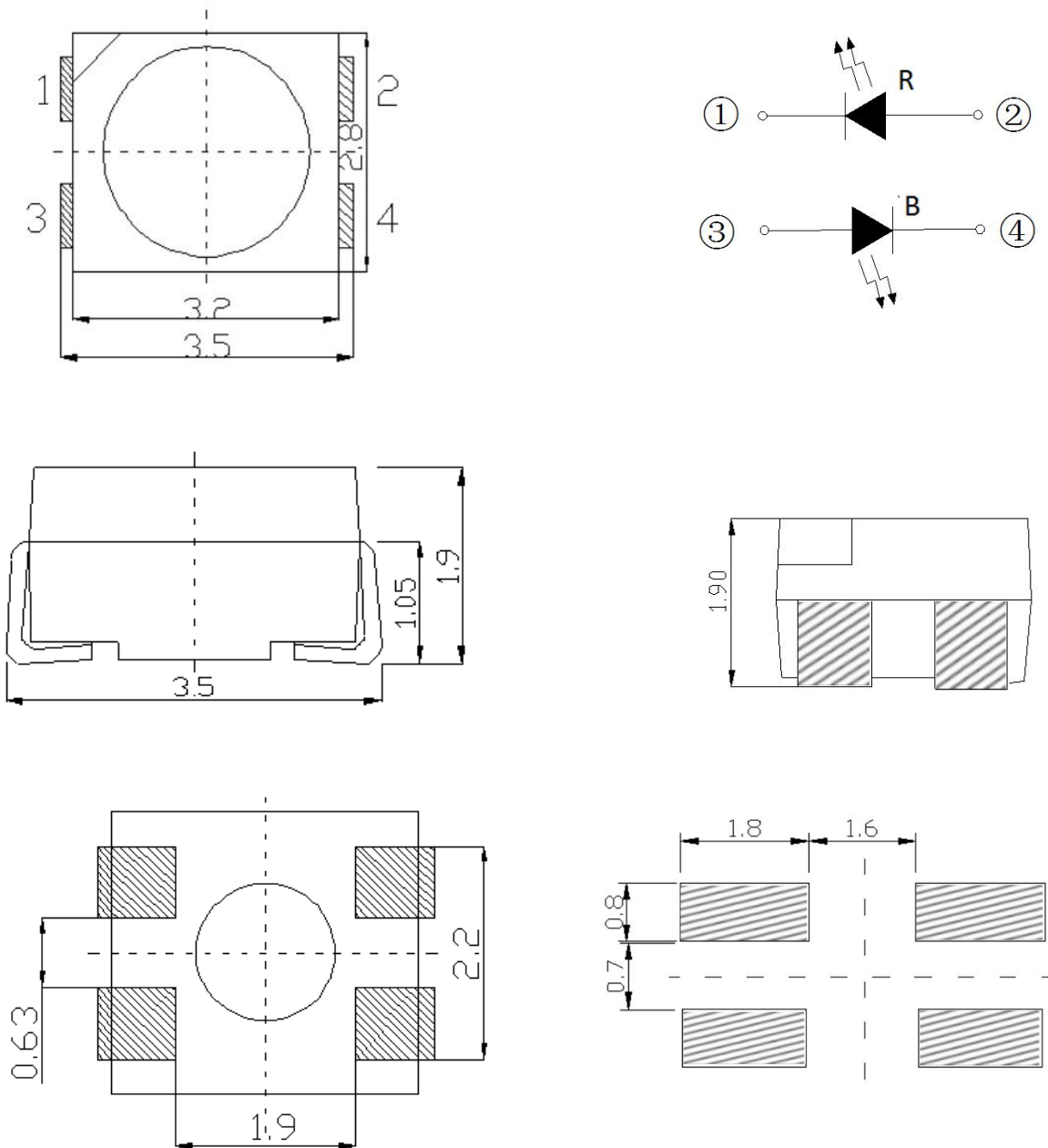
推荐焊盘尺寸 Recommended Soldering Pad
